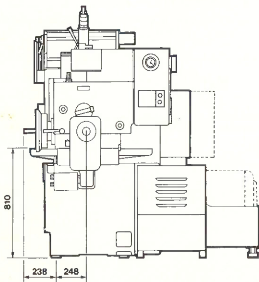
Fig. 5/1 Right side view
