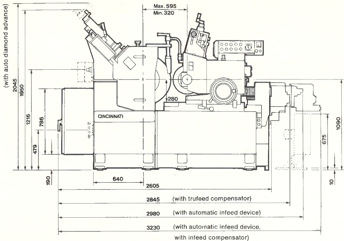
Fig. 4/1 Front view
