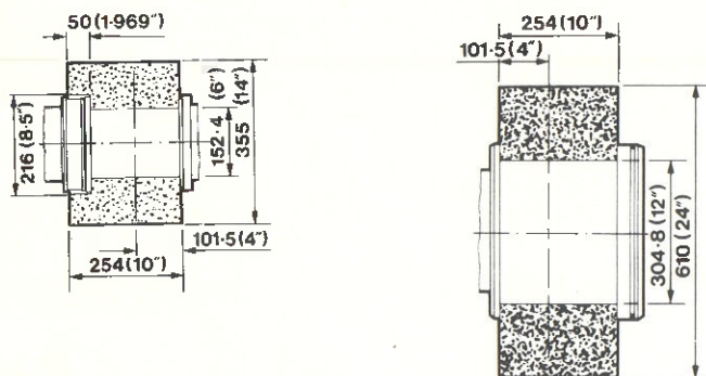
Fig. 4/1 Front view
